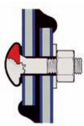
Drawing bolting / sealing of the segment sheets
