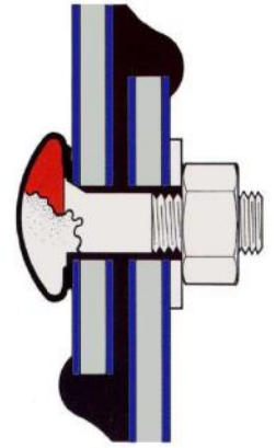
bolting / sealing of the segment sheets
