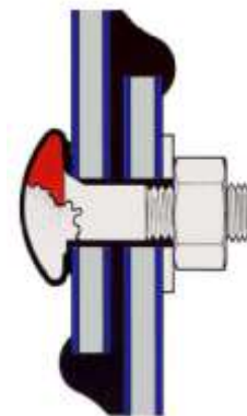
bolting / sealing of the segment sheets
